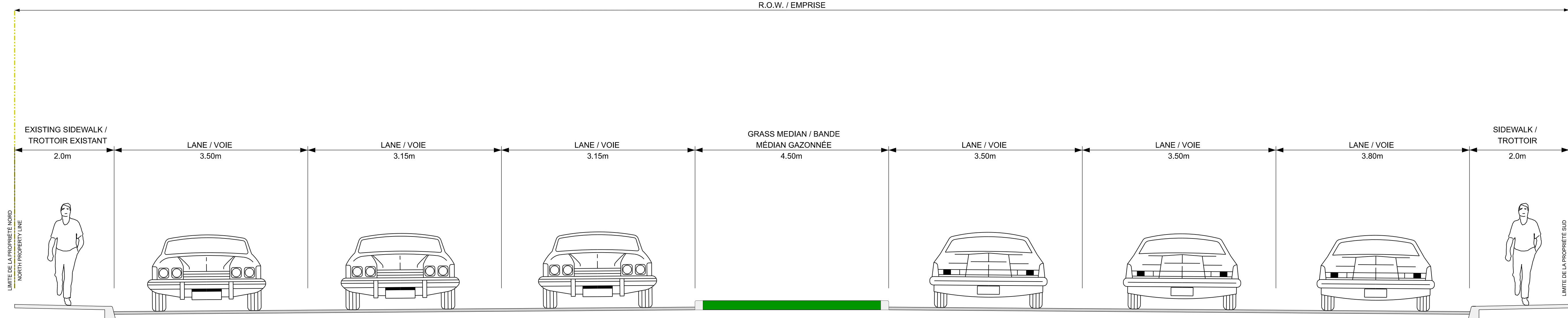
TYPICAL SECTION / COUPE TYPIQUE - AVENUE CARLING AVENUE B-B
