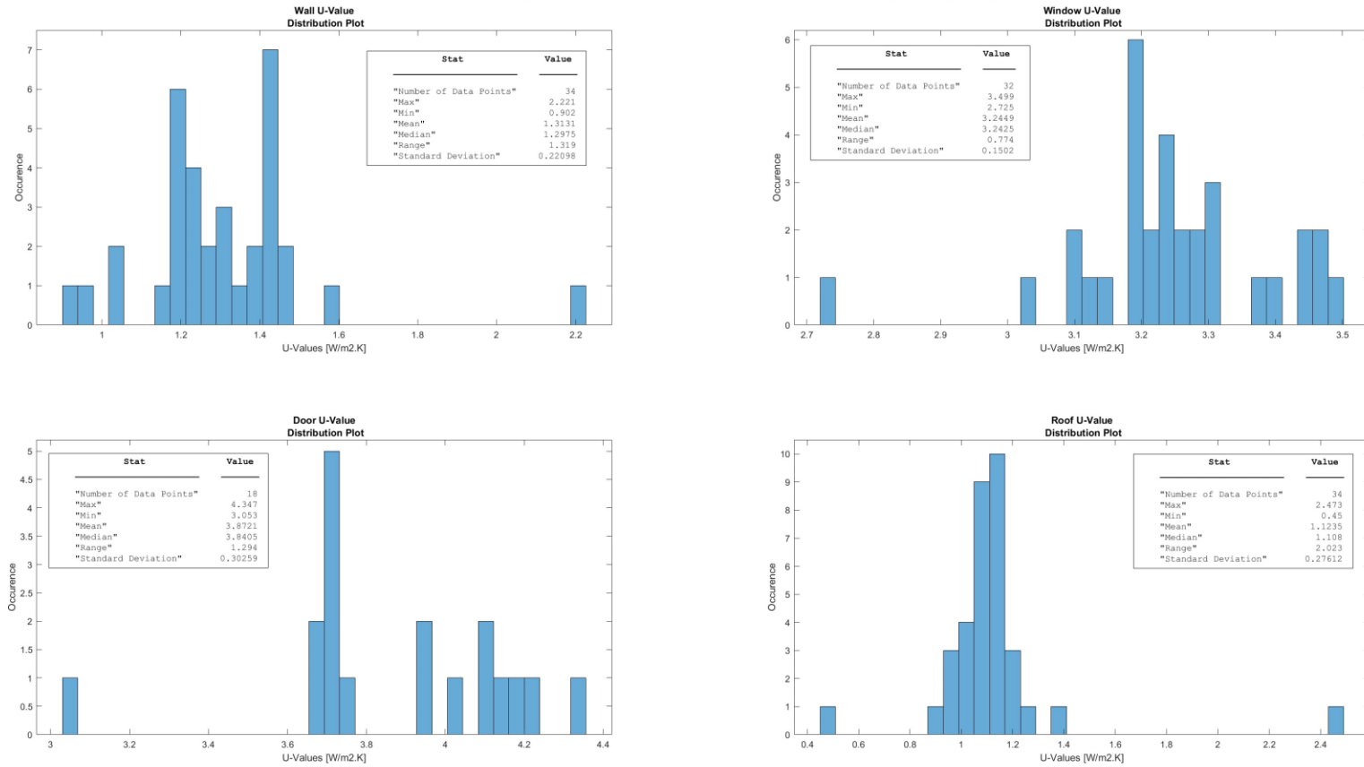
Figure 28: Summary of U-Values in Downtown Ottawa Buildings – Vintage Group 4
