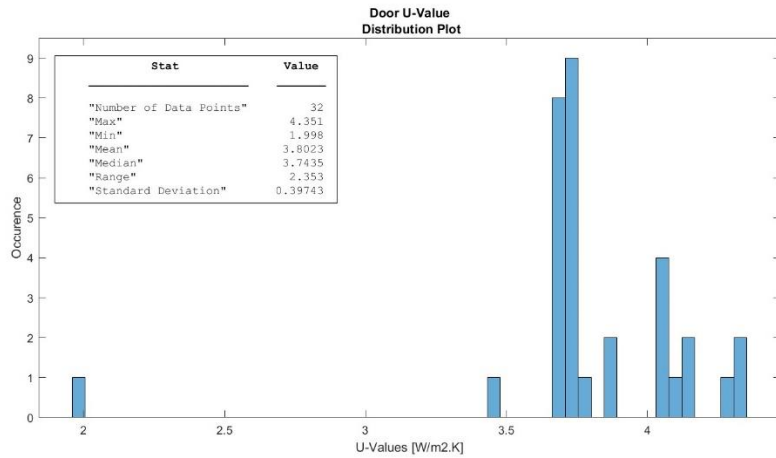
Figure 29: Summary of U-Values in Kanata Buildings
