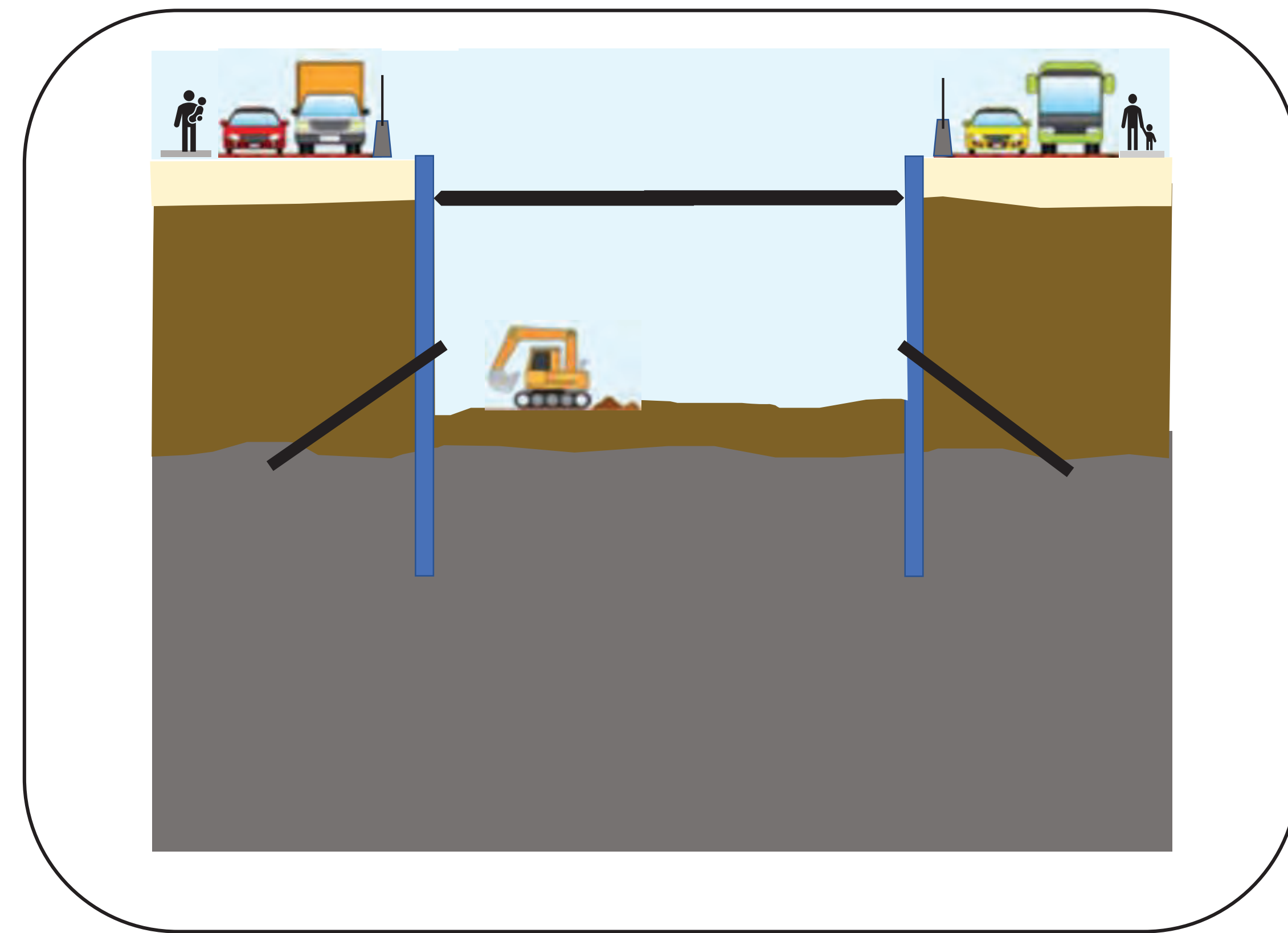
4. Excavate "CUT" and Install additional support
