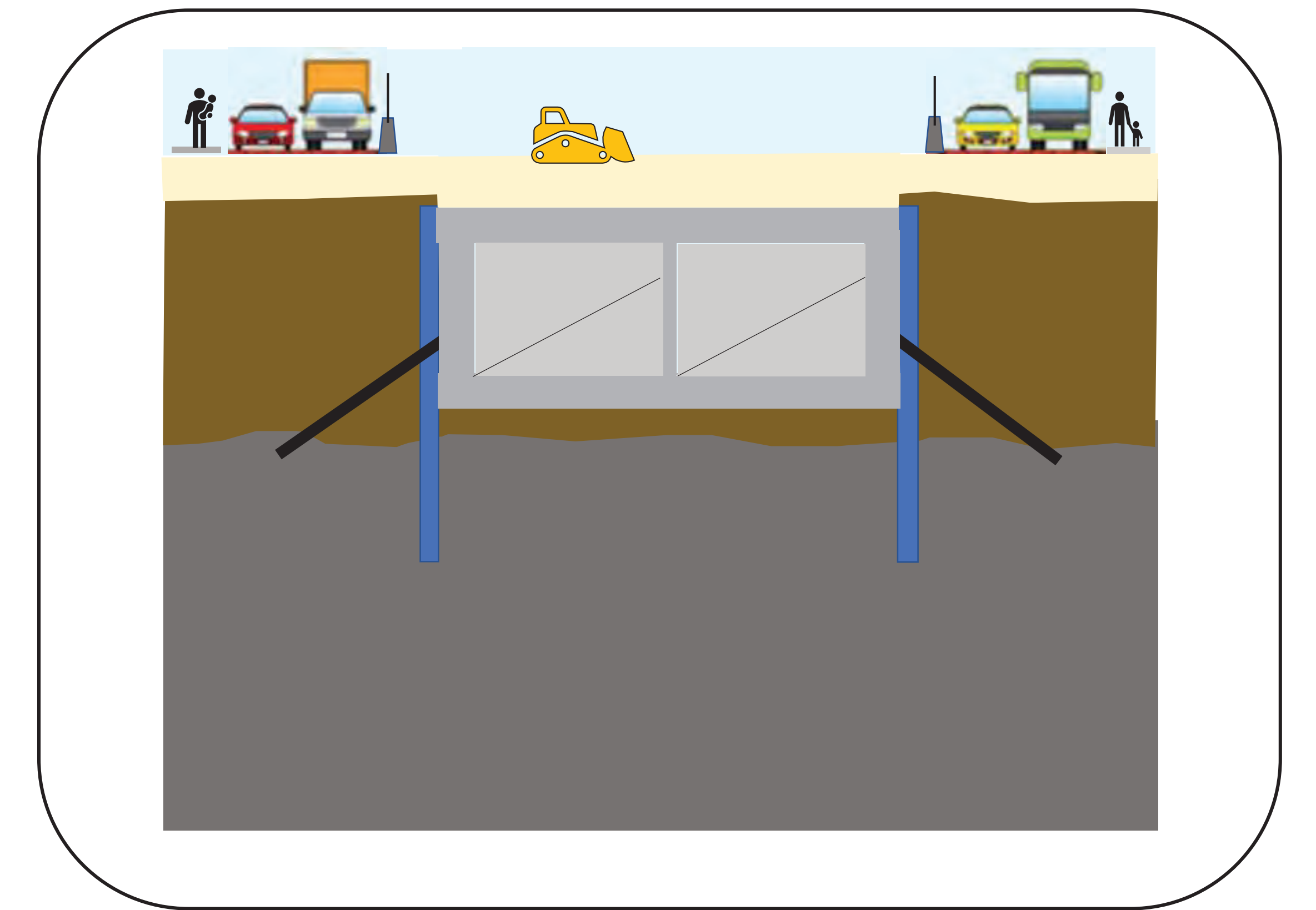
6. Remove Supports and Install "COVER" to grade
