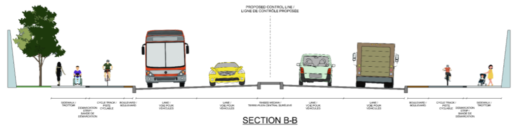
SECTION B-B
