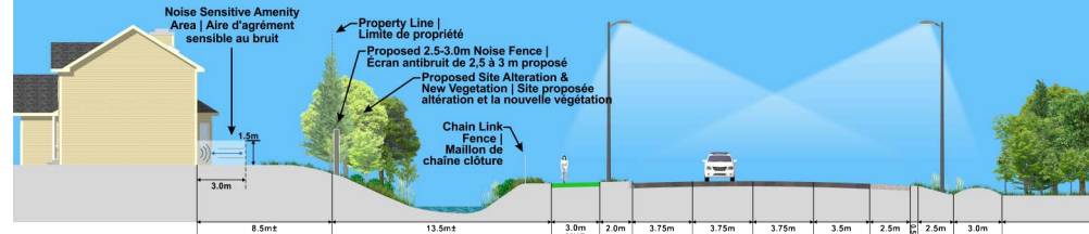
Option 1: Mitigate with Noise Fence at Property Line
