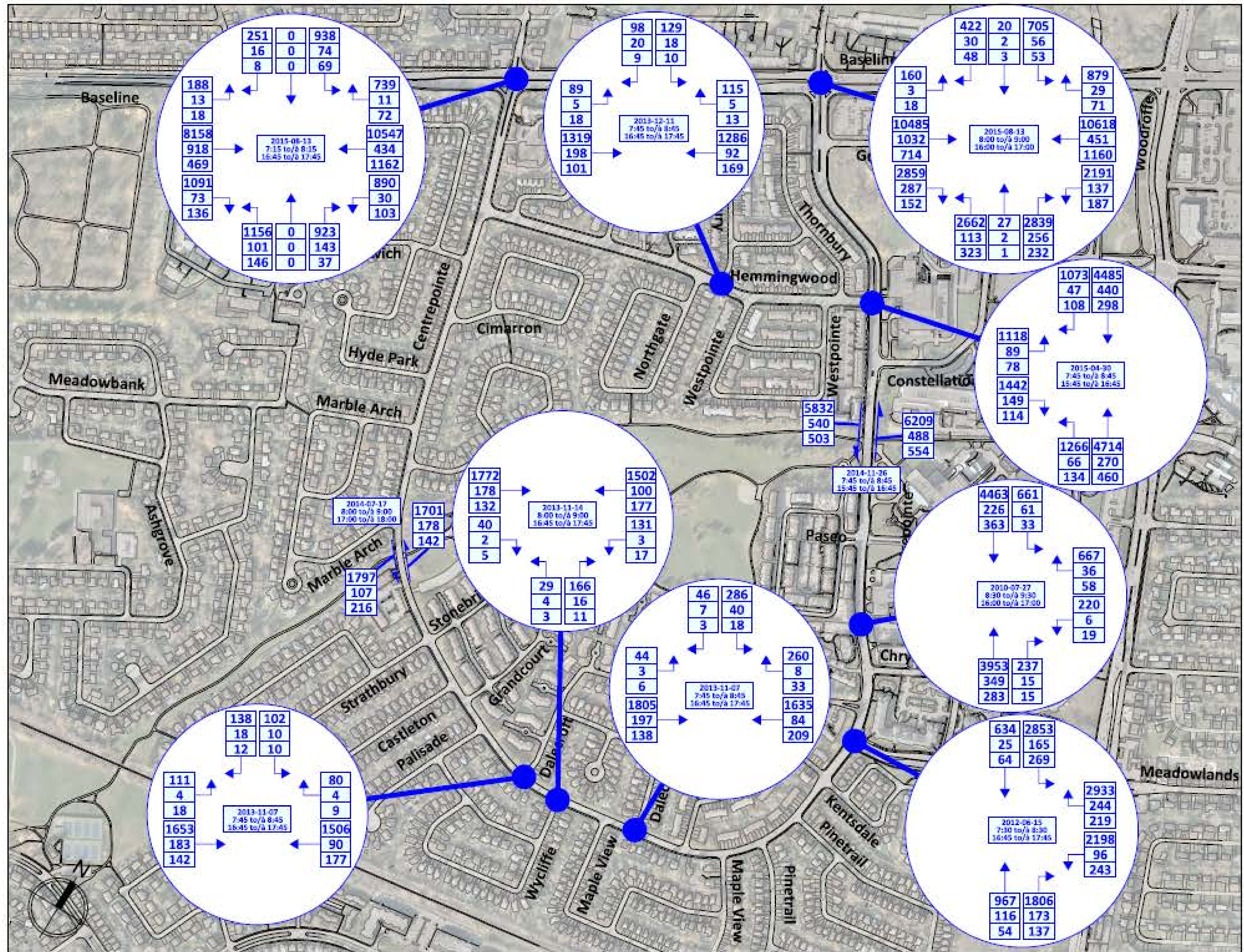
CENTREPOINTE DRIVE AND HEMMINGWOOD WAY AREA TRAFFIC MANAGEMENT STUDY Traffic Volumes (Vehicles)
