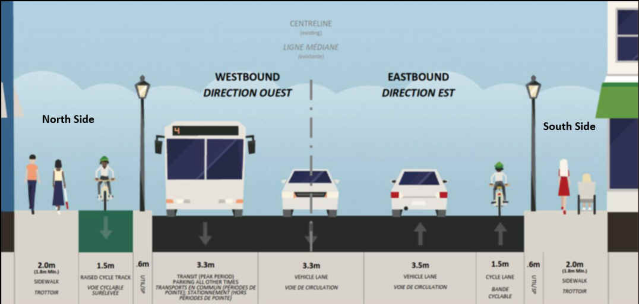
Montreal Road Functional Planning Study Proposed Montreal Road Cross-Section between Vanier Parkway and St. Laurent Boulevard
