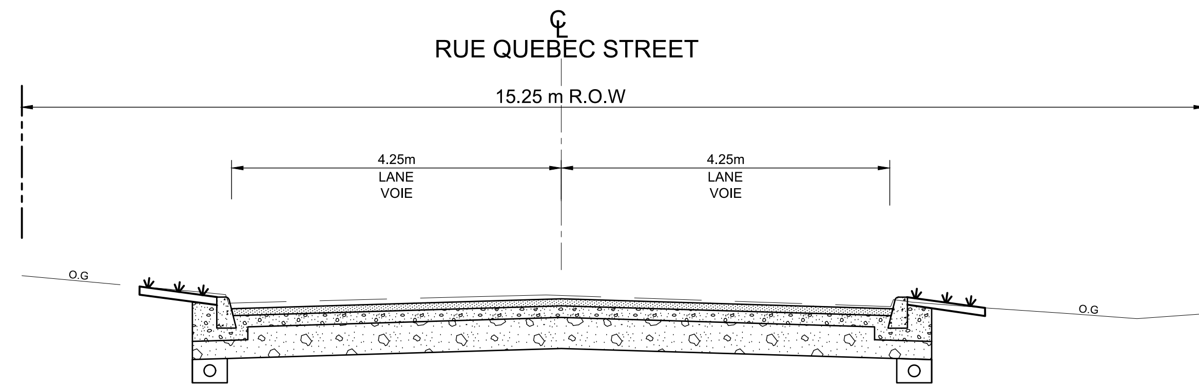
TYPICAL ROADWAY CROSS SECTION COUPE TYPE RUE QUEBEC STREET
