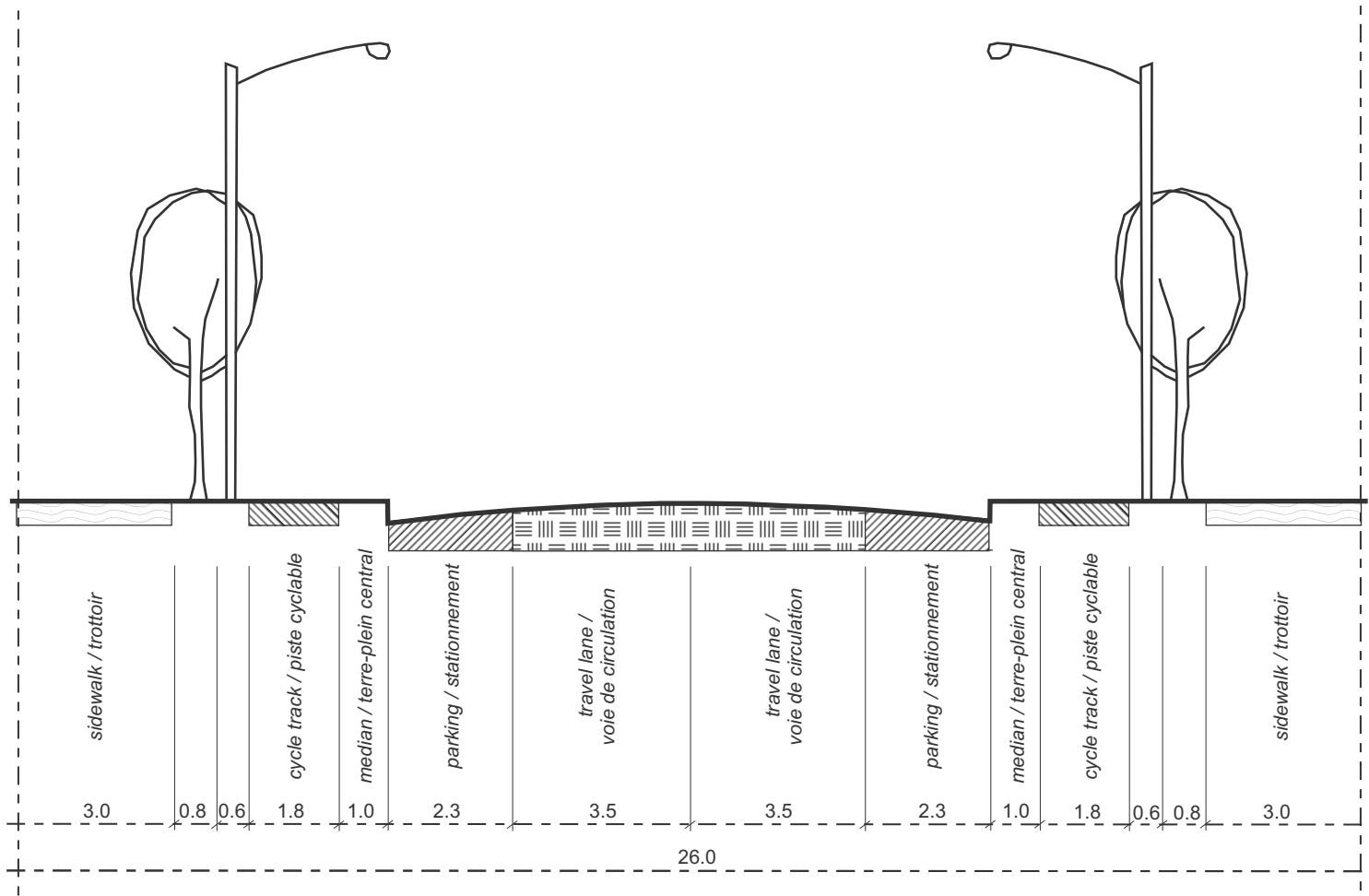
APPENDIX 2 RIVERSIDE SOUTH - CORE AREA MAIN STREET X-SECTION
