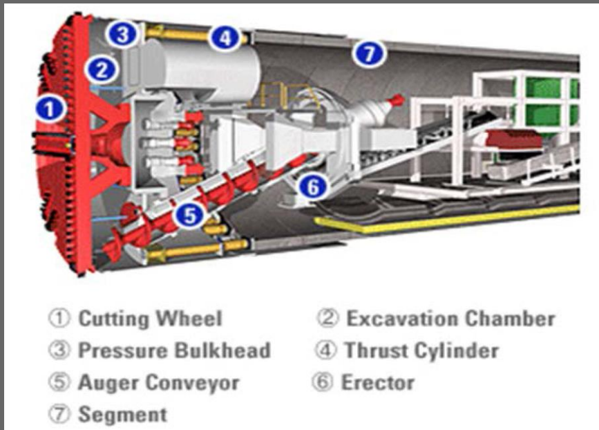
TBM Schematic
