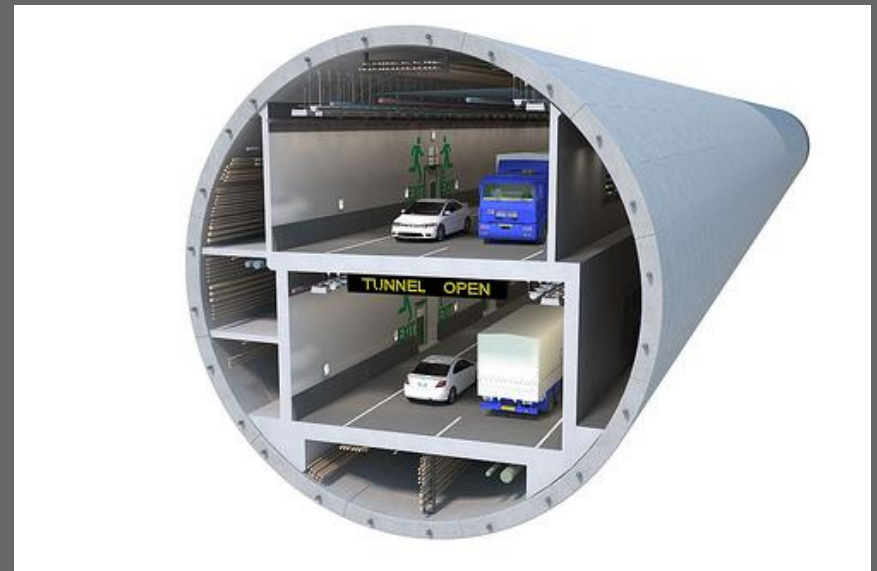
Example Double-Deck Structure
