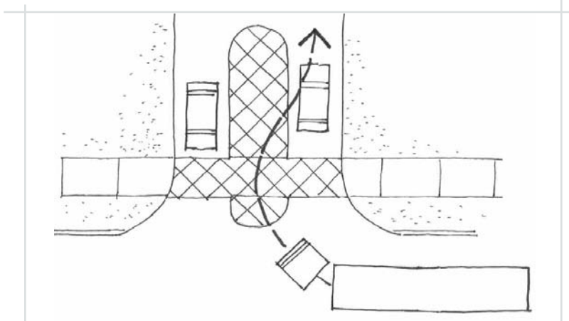
Figure 11: The car entrance and pedestrian crossing are clearly defined; flush contrasting paving allows for tanker truck turning.
