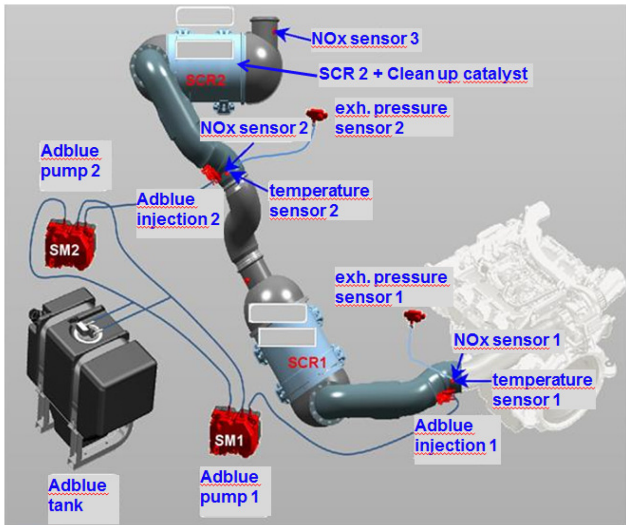
Figure 2: Overview of the Tier 4f (final) SCR system
