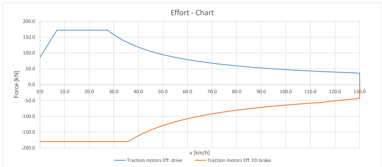
Figure 3: Tractive effort versus speed diagram 1
