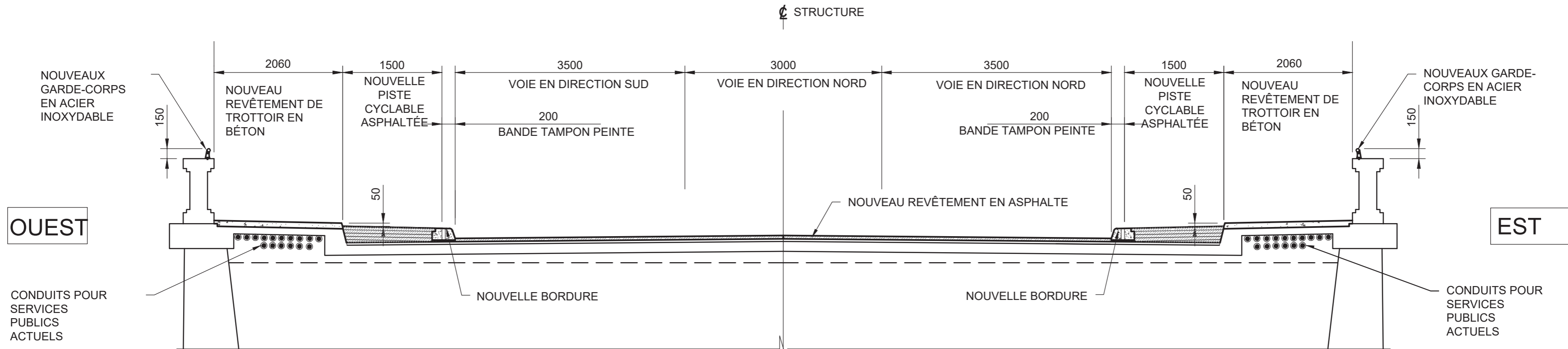
SECTION (TYPE)
