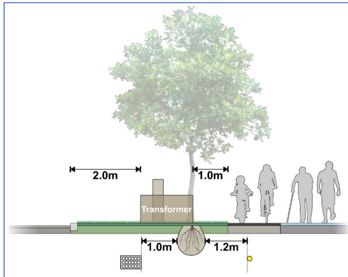
Figure 21 Surface-mount hydroelectric transformers need separation from roadways, parking, cycle-tracks and sidewalks, and tree root balls must have separation when planted (minimum of 1.0m from duct banks and 1.2m from gas main)
