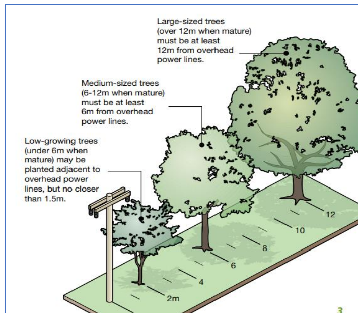
Figure 22 Tree planting restrictions near aerial utilities [source: Hydro Ottawa]
