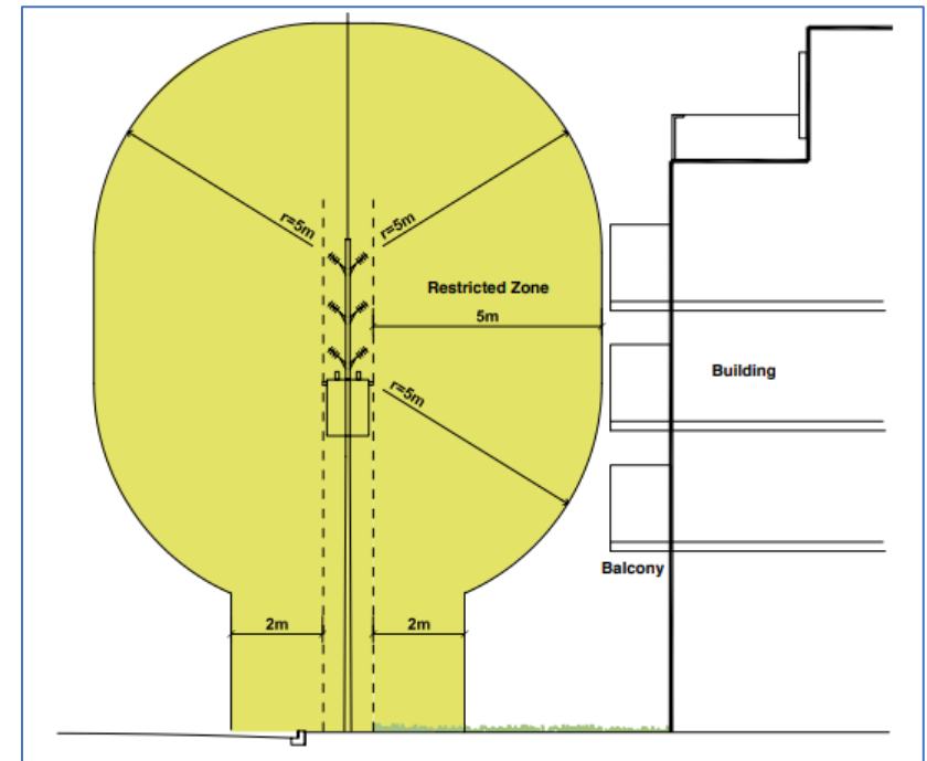
Figure 23 Building restrictions near aerial utilities [source: Hydro Ottawa]
