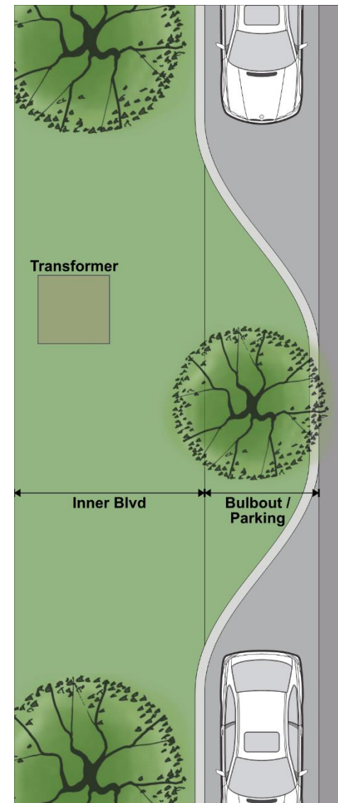
Figure 20 Bulb-outs can provide additional opportunities for other design elements
