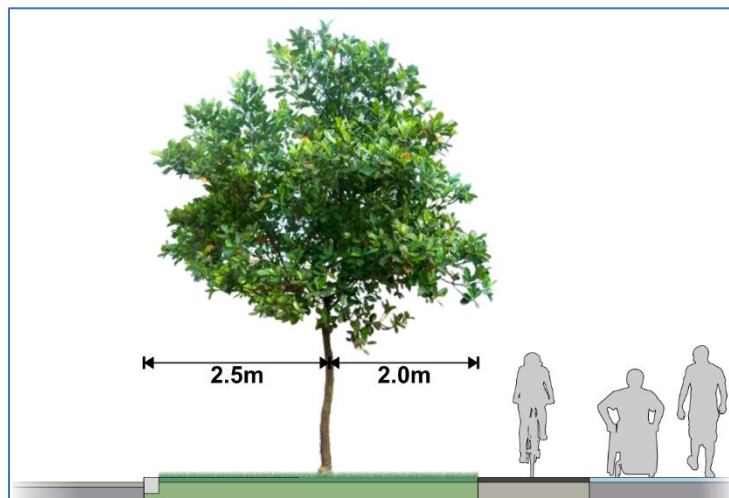
Figure 18 Offset trees from the roadway and active transportation facilities to promote growth and avoid impacts of road maintenance activities
