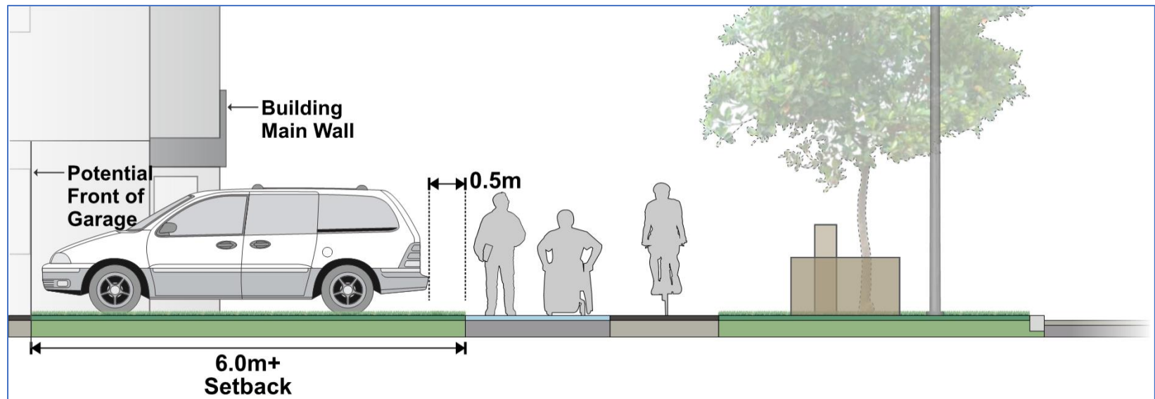
Figure 14 Driveway parking cannot be closer than 0.5m to sidewalks, cycle tracks, or curb
