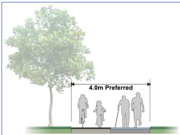
Figure 17 Sidewalk and cycle track shown in a bundled, side-by-side arrangement
