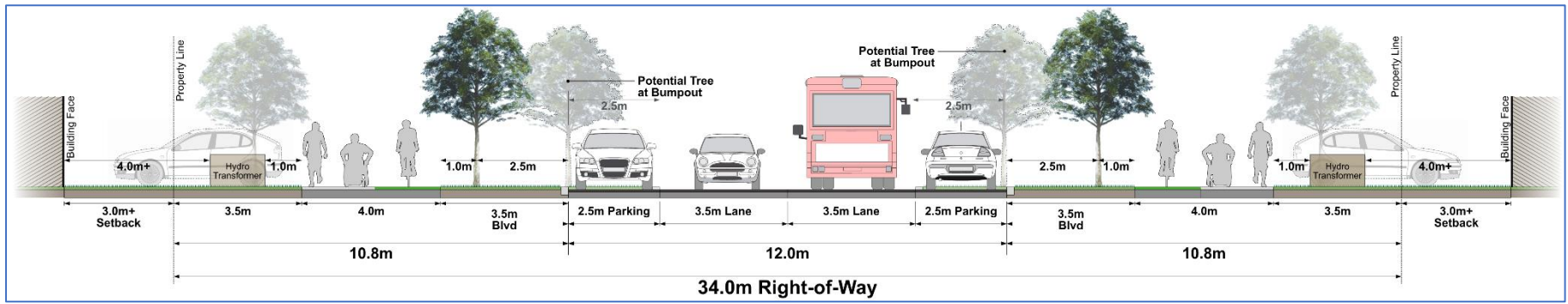
Figure 15 Demonstration of Wide, Unrationalized Right-of-Way Design
