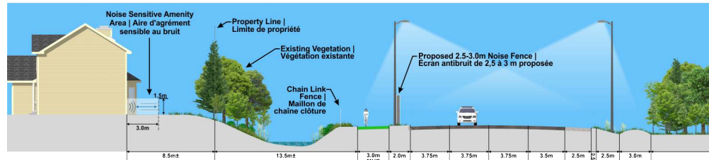
Option 3: Mitigate with Noise Fence at Road Edge
