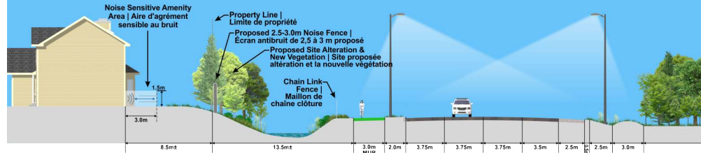
Option 1: Mitigate with Noise Fence at Property Line
