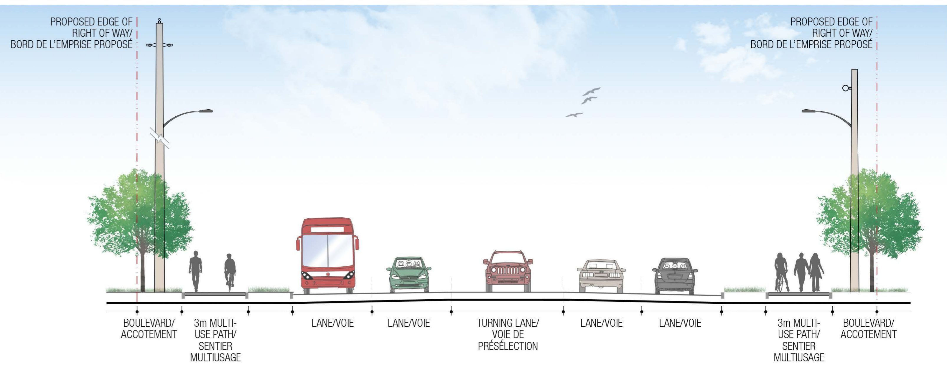
SECTION B-B
