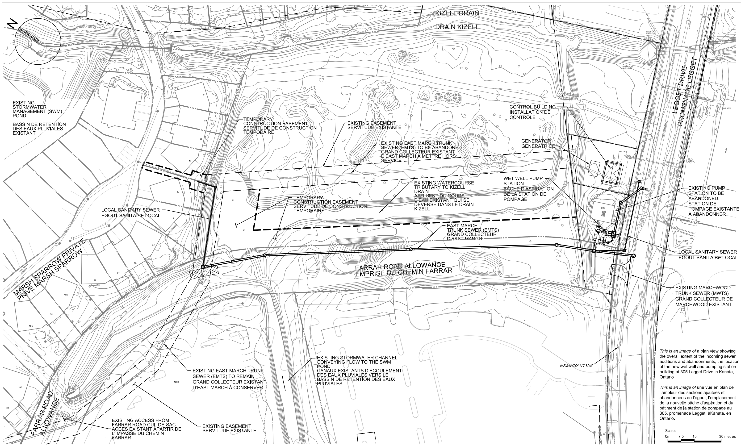
MARCH ROAD PUMP STATION DIVERSION PROJECT SITE PLAN SHOWING SEWER MODIFICATIONS
