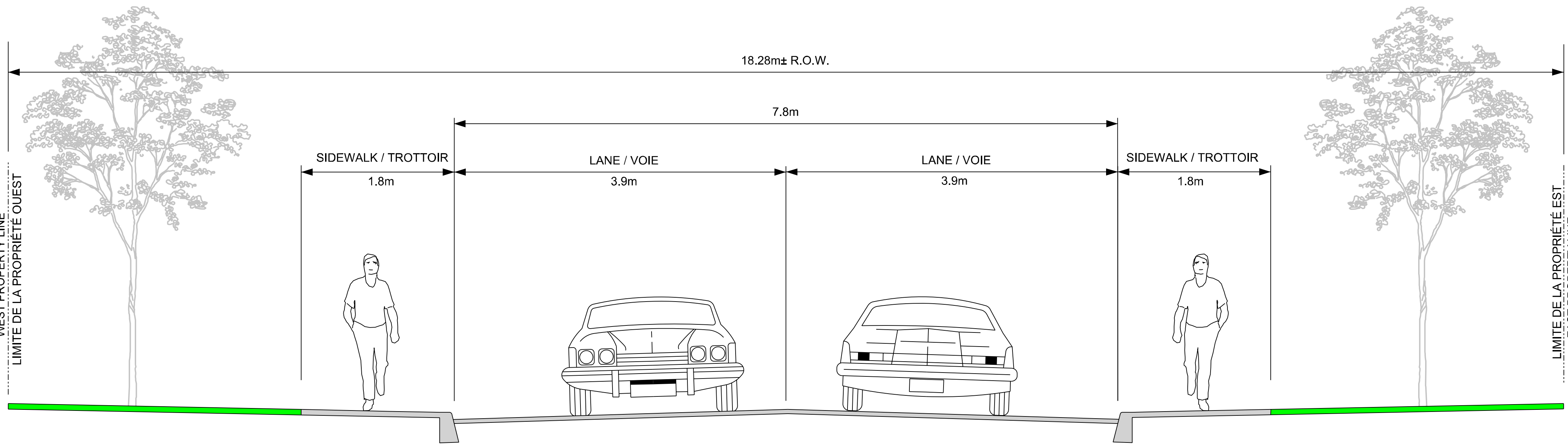
TYPICAL CROSS SECTION - RANGE ROAD COUPE TYPIQUE - CHEMIN RANGE
