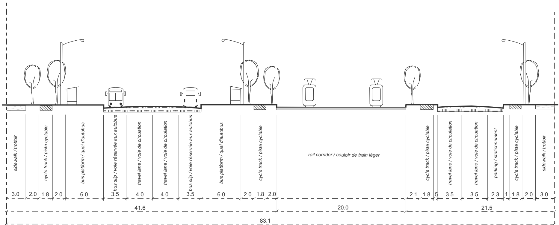
APPENDIX 3 RIVERSIDE SOUTH - CORE AREA TRANSIT STREET X-SECTION (West of Limebank Road)
