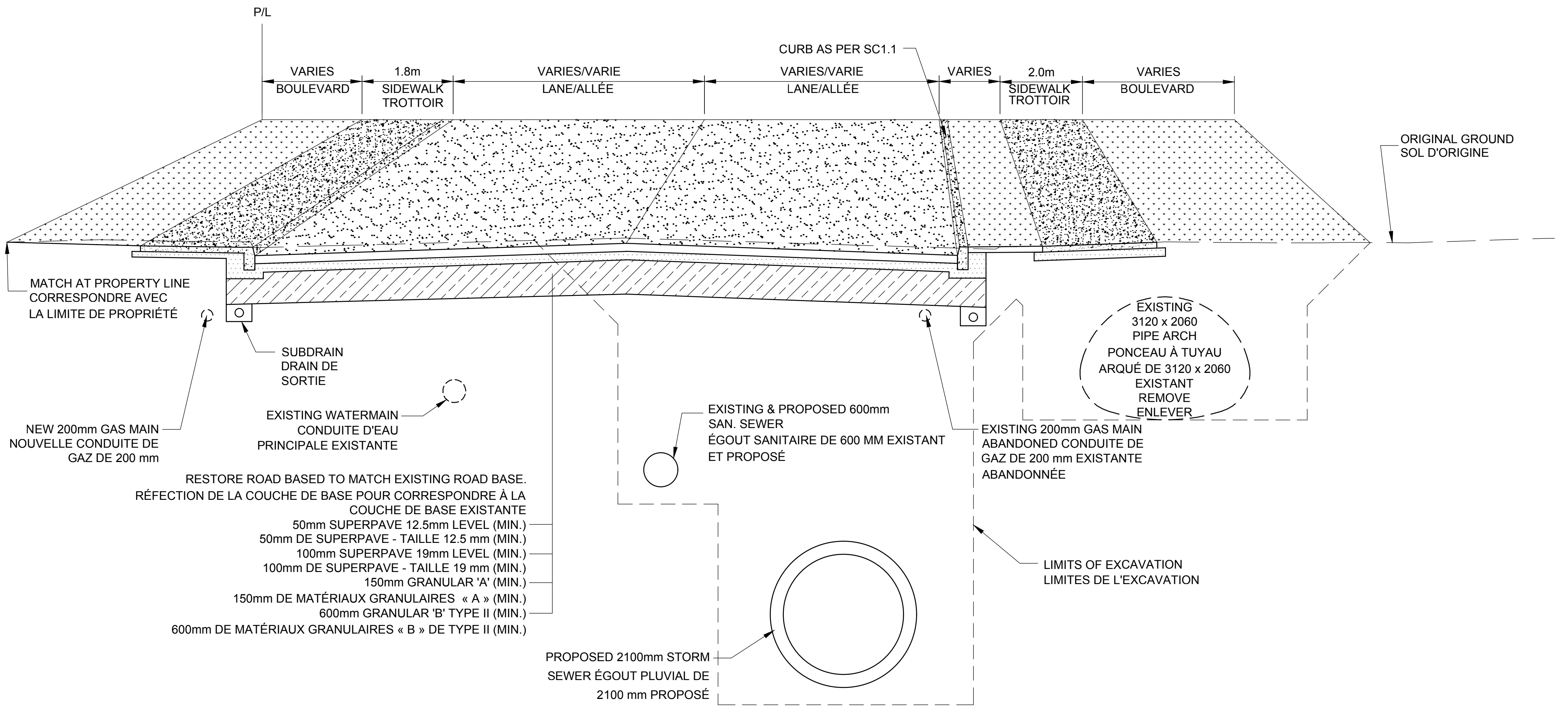
ST. LAURENT BOULEVARD TYPICAL SECTION/SECTION TYPE DU BOULEVARD ST-LAURENT
