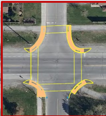
Pedestrian landing pads and missing crosswalk at Johnston East
