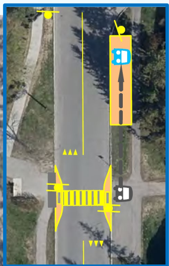
PXO type D with bulb-outs and bus stop re-location
