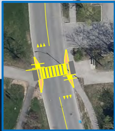
PXO type D with bulb-outs
